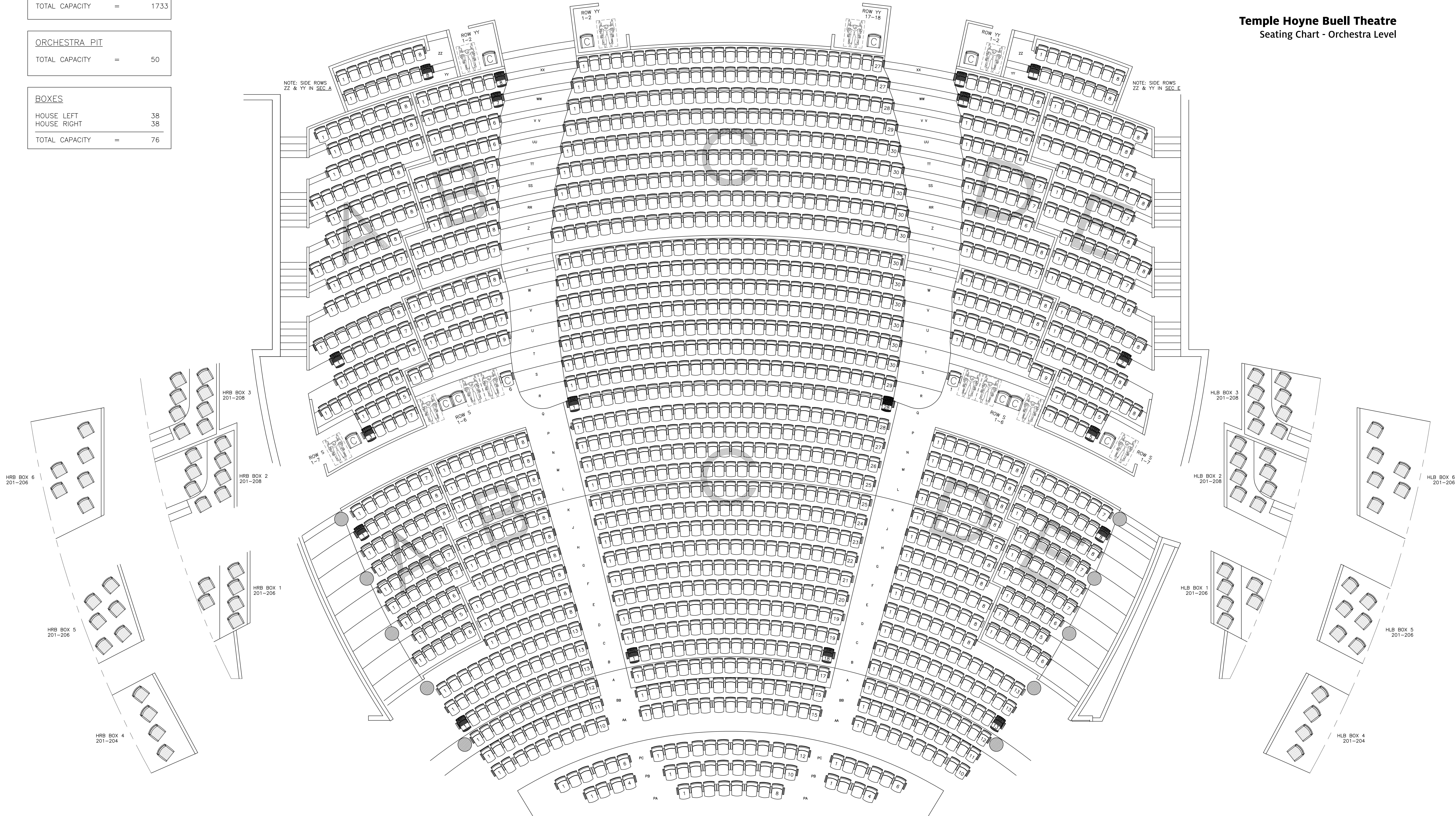
PLAN VIEW: ORCHESTRA SCALE: 3/16"=1'-0"
